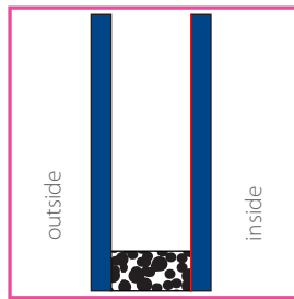
Double glazing packet, safety glass on both sides Ug=1,1 (EN673) 4 ESG /16ar/4 ESG, aluminium distance spacer
