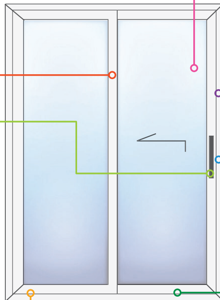
Double glazing packet, safety glass on both sides Ug=1,1 (EN673) 4 ESG /16ar/4 ESG, aluminium distance spacer
